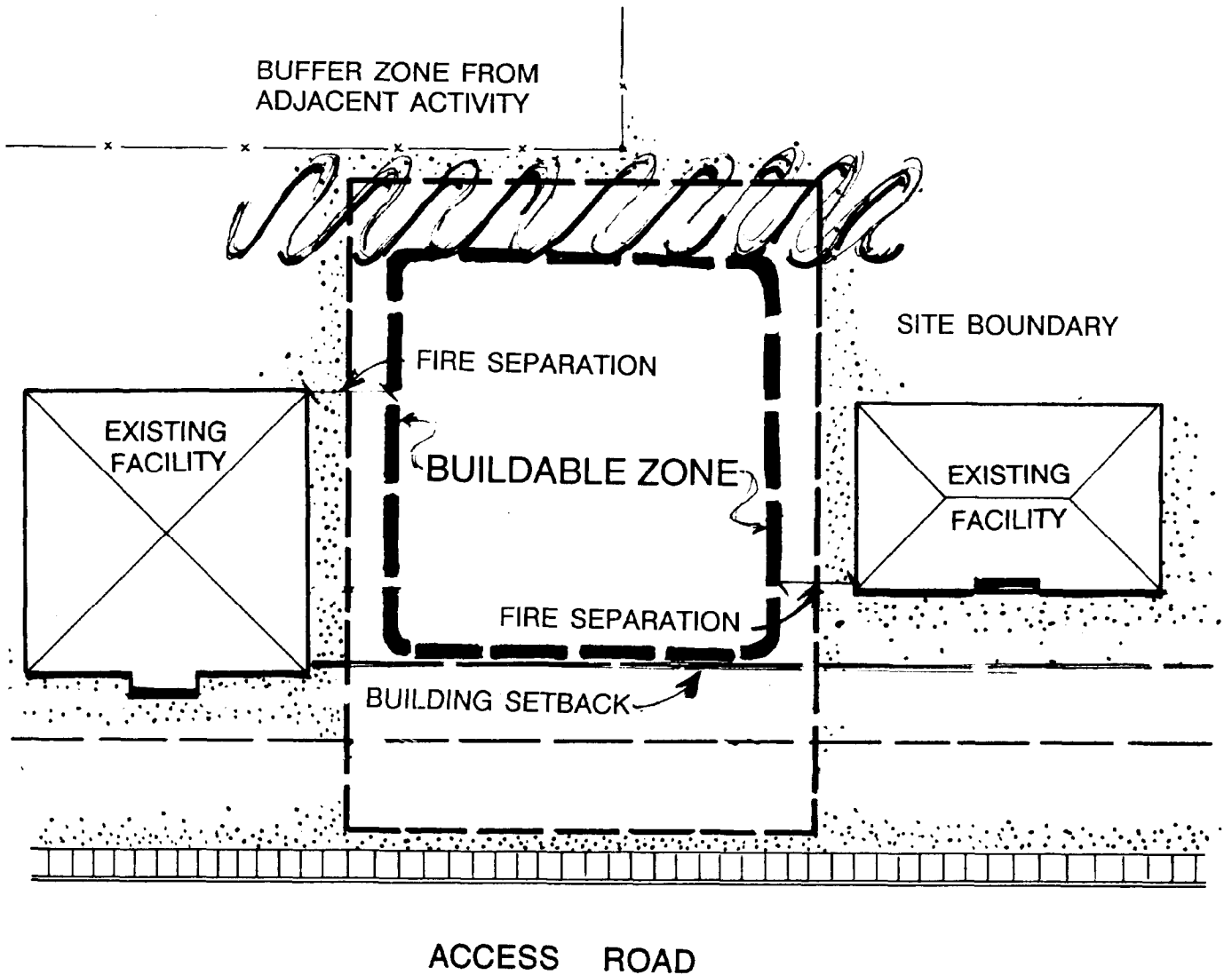
Figure 4-2. Buildable Zone.
